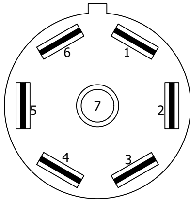
VIEW LOOKING INTO HOST VEHICLE AND SAFETY HITCH BASKET CONNECTOR
