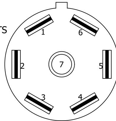
VIEW LOOKING INTO 7-PIN CABLE
